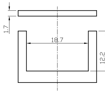
PANEL CUT-OUT
